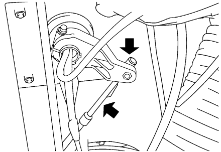
1 Adjuster
