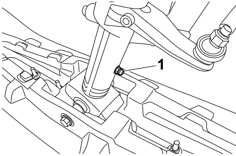
1. Grease nipple
