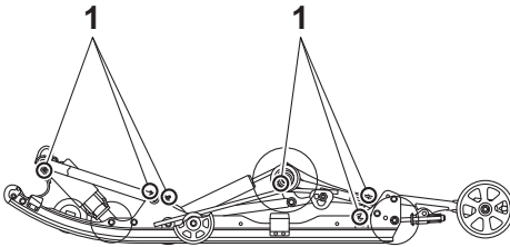
1. Grease nipple
