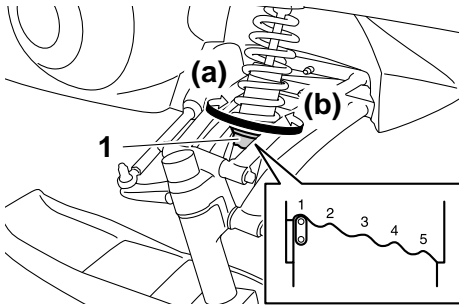
1. Spring preload adjusting ring
