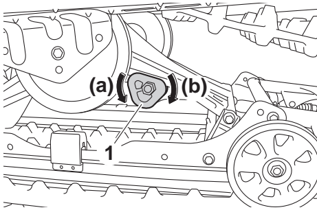
1. Spring preload adjuster
