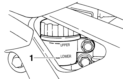
1. Merkstreep minimumniveau
