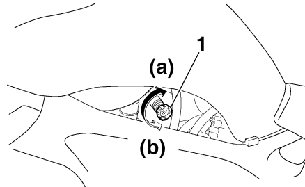
1. Stationair stelschroef
