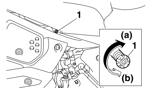
1. Stationair stelschroef
