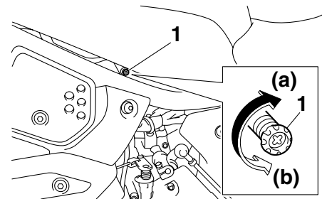
1. Stationair stelschroef
