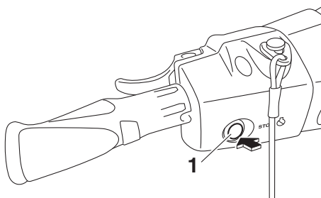
1 Motor-Stoppsschalter
