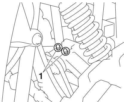
1. Grease nipple
