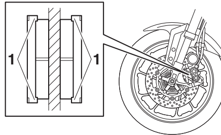
1. Slijtage-indicator remblok
