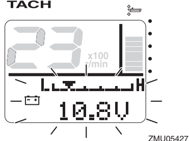
TACH
