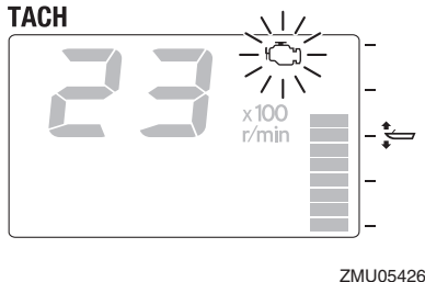
TACH
