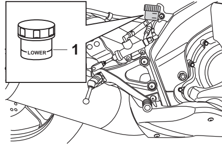
1. Merkstreep minimumniveau
