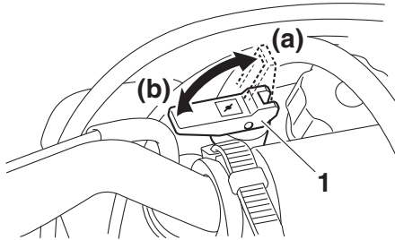
1. Chokehebel “|⌘”
