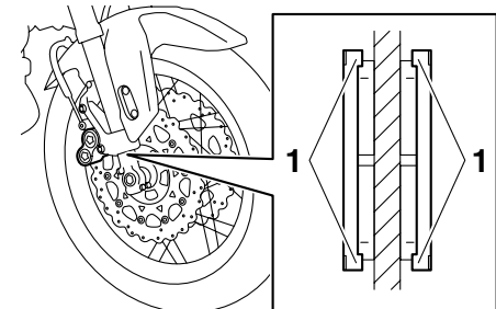
1. Slijtage-indicator remblok
